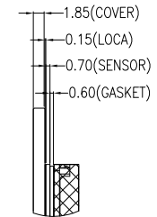
DETAIL B (SCALE 2:1)
